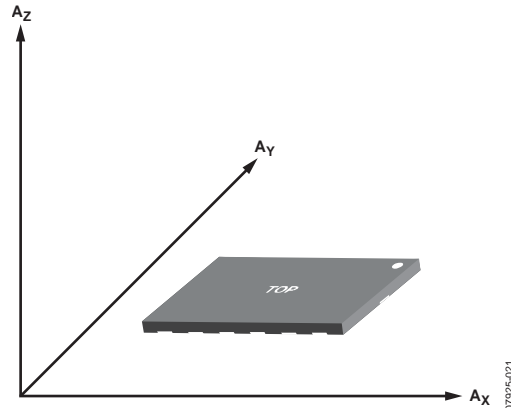
Figure 56. Axes of Acceleration Sensitivity (Corresponding Output Voltage Increases When Accelerated Along the Sensitive Axis)
